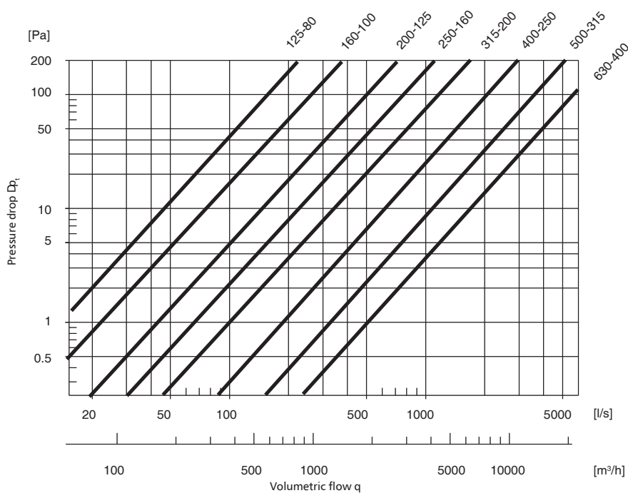
2 reduction stage
